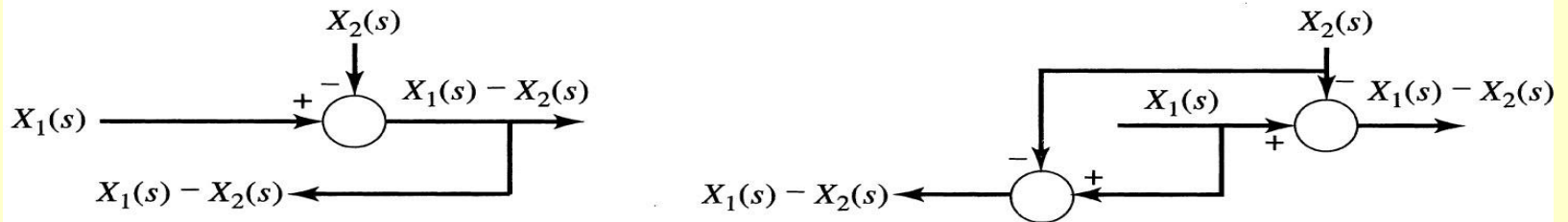
(g) Moving a pickoff point behind a summation
