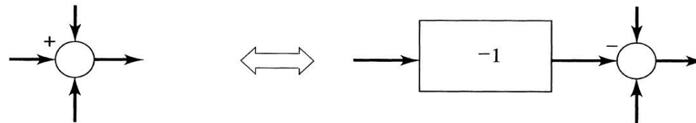
(b) Changing a summer sign
