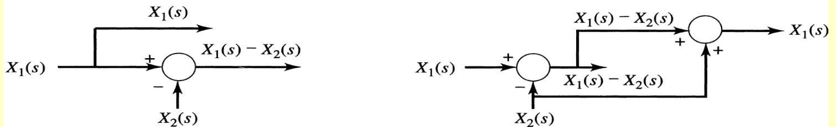
(h) Moving a pickoff point forward of a summation
