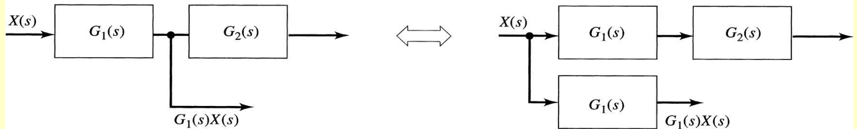
(c) Moving a pickoff point back
