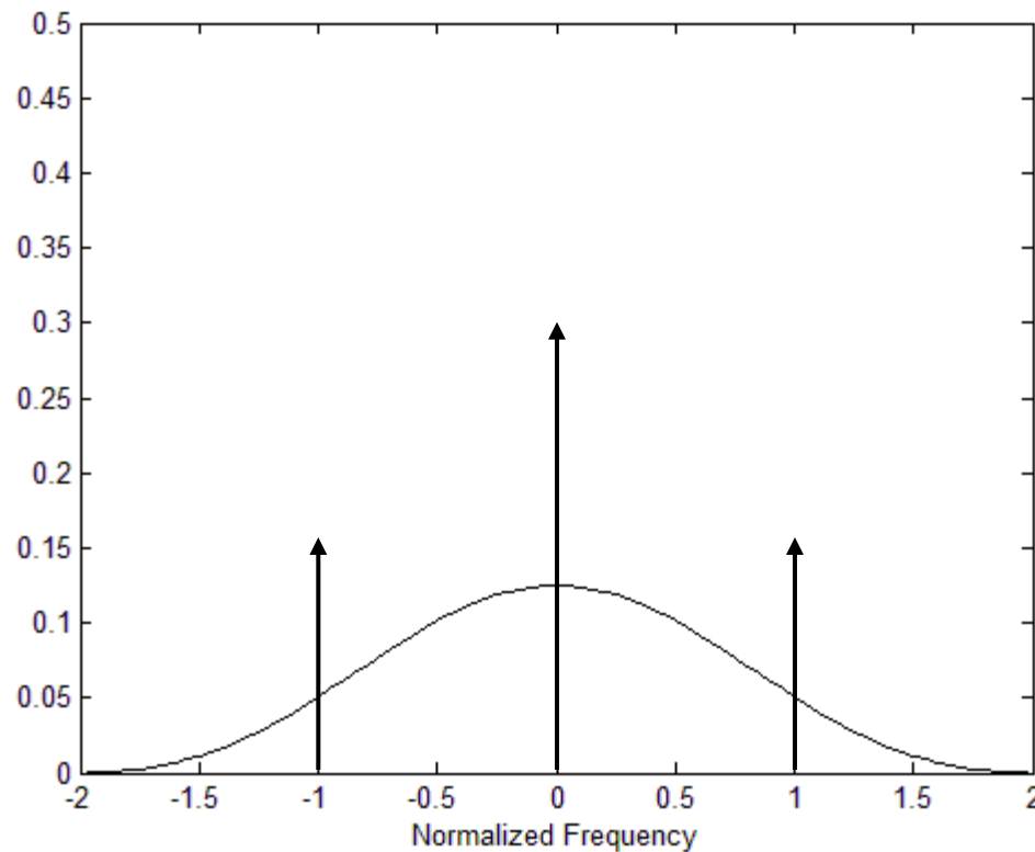
PSD of Unipolar RZ
