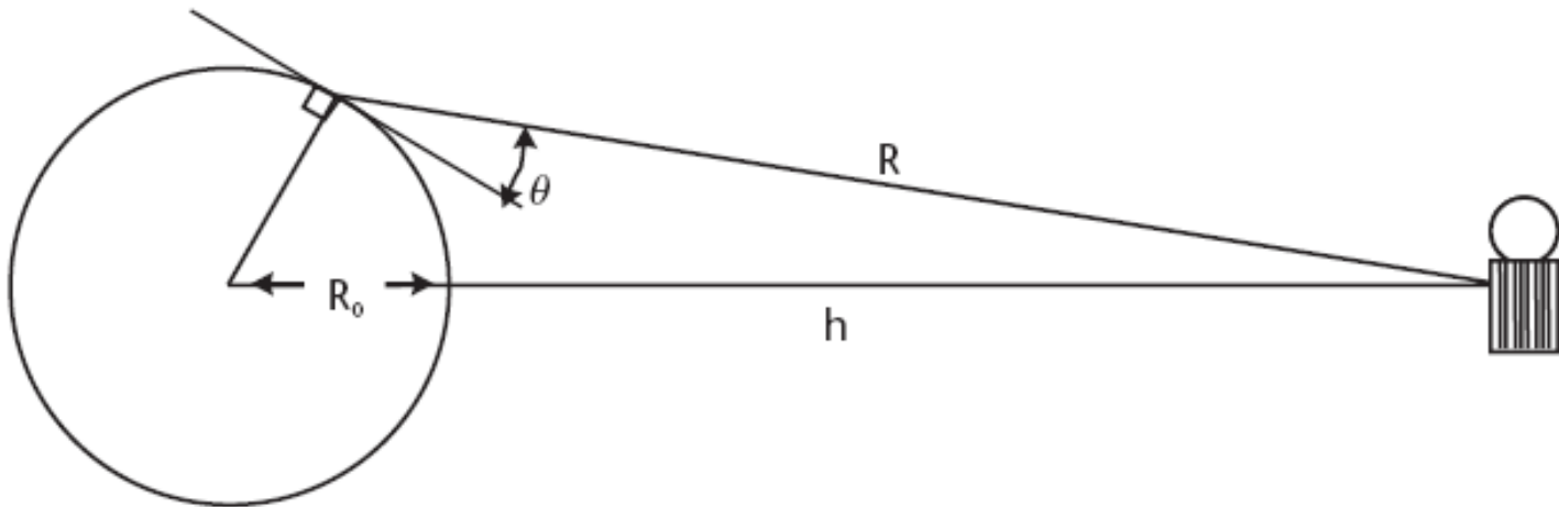
Figure 2.2 Definition of the slant range distance, R , between the Earth station and the GEO satellite. The Earth station elevation angle, \theta , is with respect to the local horizon.
