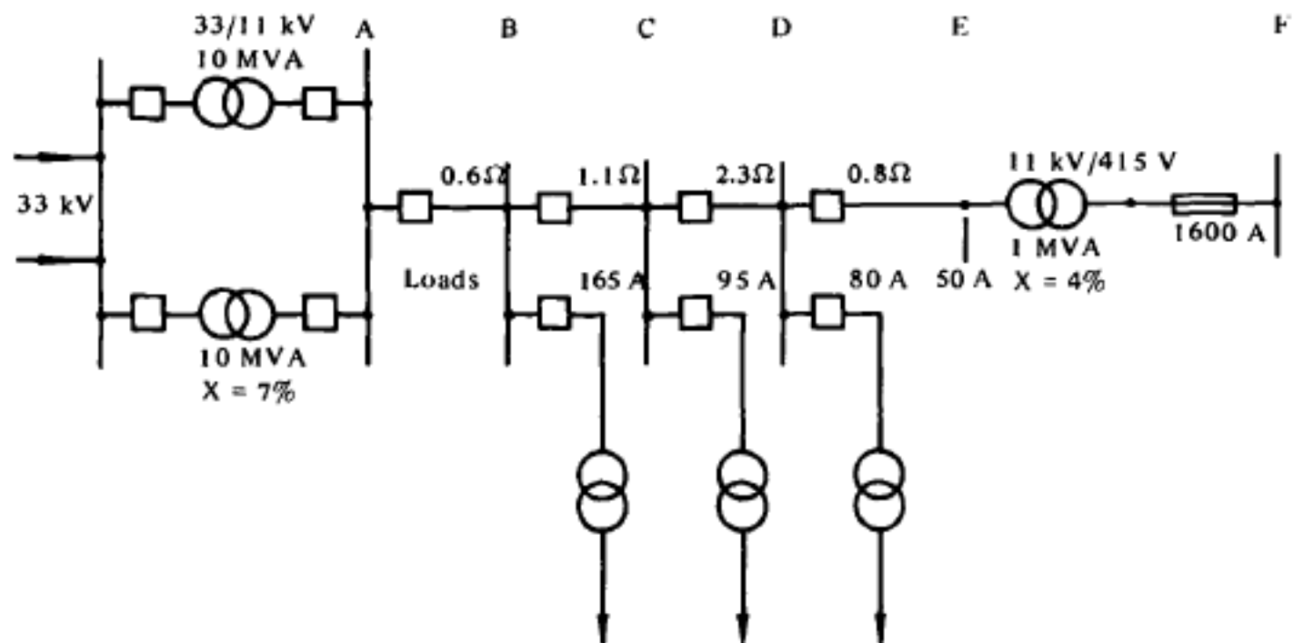
Fig. 8.3.2.2 11kV radial system; data for grading calculation
