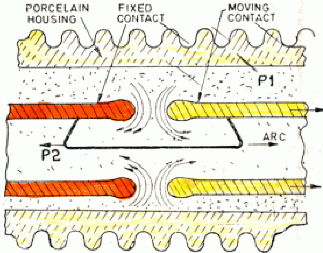
(b) Double axial flow.
