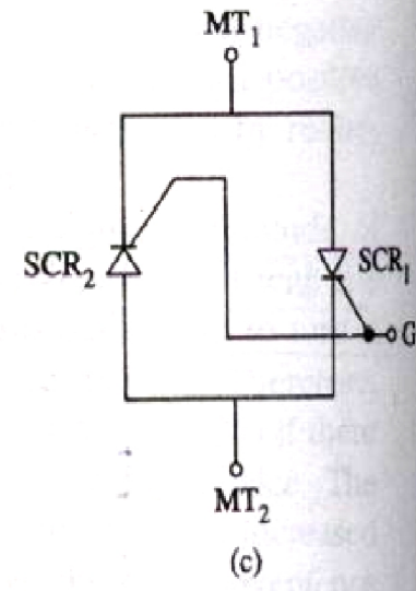
SCR equivalent circuit
