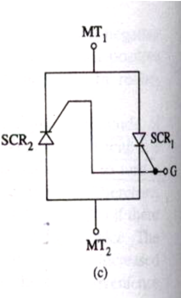
SCR equivalent circuit
