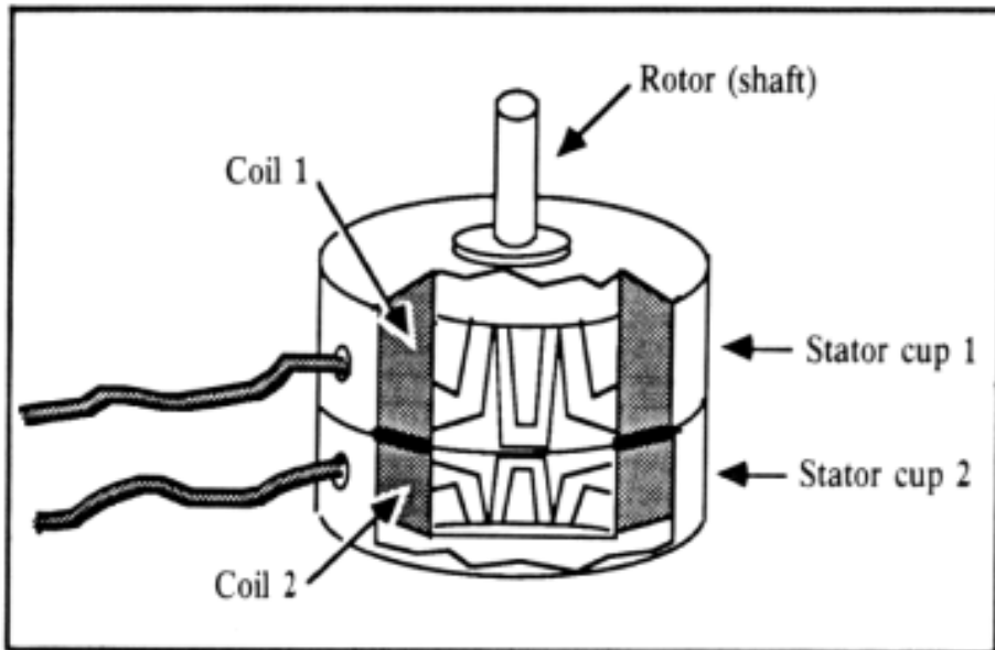
Fig. 14-2. Inside a four-phase stepper motor. Note the two sets of coils and stators. The four-phase stepper is really two motors in one.
