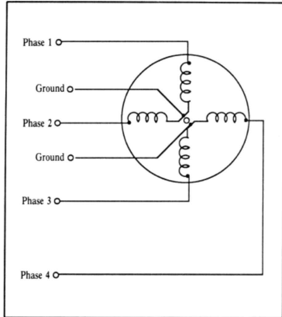
Fig. 14-3. The wiring diagram of the four-phase stepper. The ground connections may be separate or combined.
