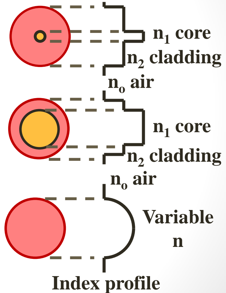
Multimode graded-index Fiber
